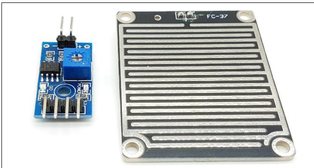
Fig 1. Rain Control Module – LM393 Comparator
